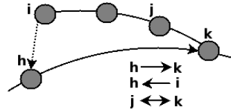
Figure 1. The relaxed-ring architecture
