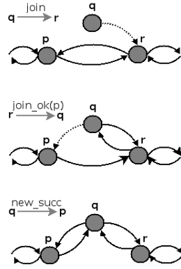
Figure 2. The join algorithm.
